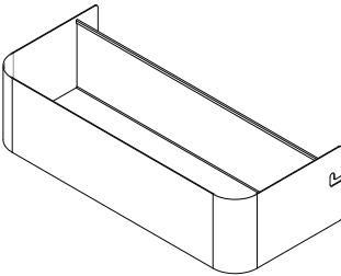
METAL WALL PLANTER - 24" Materials: Steel & MDF Dims: 6"H x 23.635"W x 8.095"D 251056
