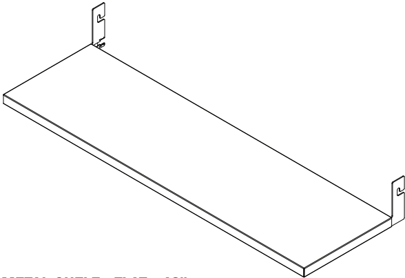
METAL SHELF - FLAT - 48" D 14" W 48" H 1 ¼" Material: Steel 251005E
