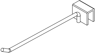
HANGRAIL PEG HOOK - 6" W 1/2" H 1/4" L 6" Material: Steel 251036
