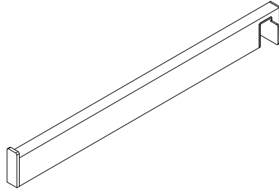
FACEOUT - HANGRAIL - 14" W 1/2" H 1 1/4" Material: Steel To be used on Shallow Hangrails 251035
